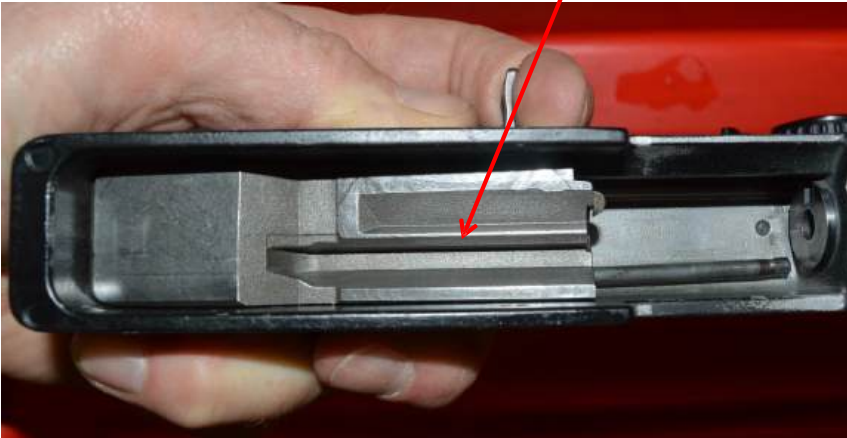
Bolt inserted but not fully located.
